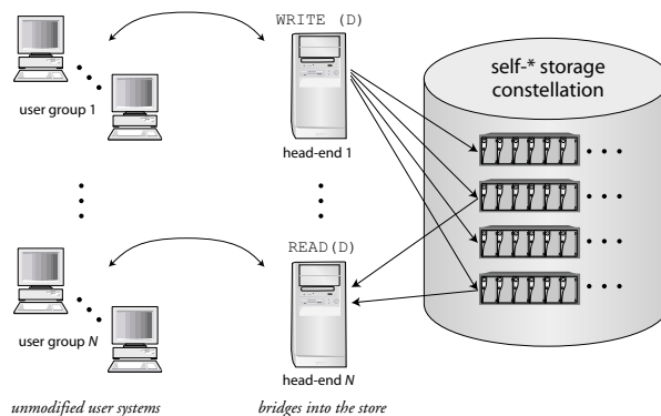
Figure 3: “Head-end” servers bridge external clients into the self-* storage constellation.
